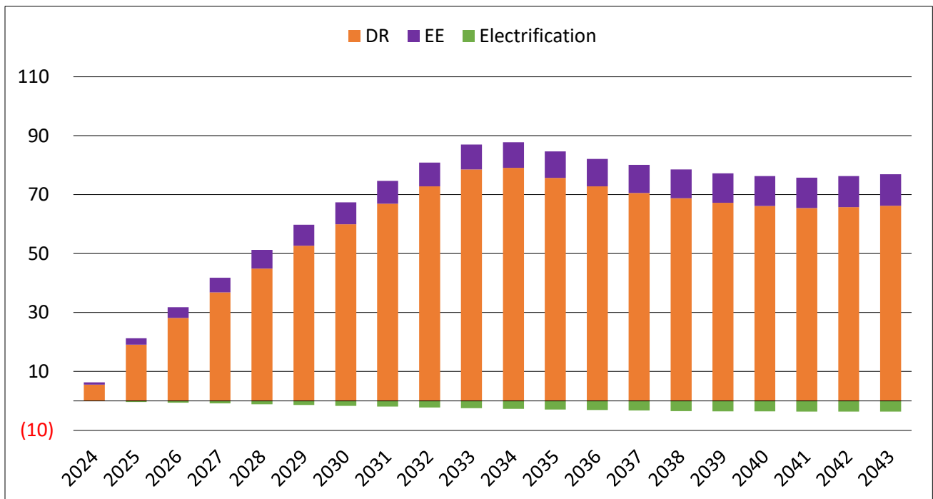
Figure 4-12: 25+ MW DSM by Resource Type, Winter Season (MW)
